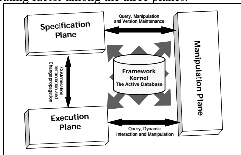
Figure 2. SpEM framework
