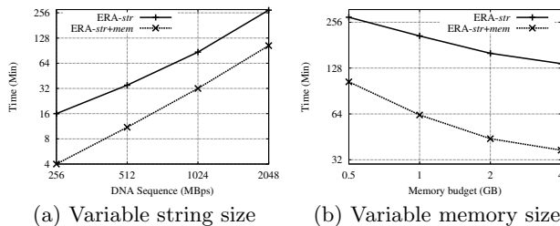
Figure 7: Serial execution time of horizontal partitioning methods; DNA dataset. (a) 512MB RAM; (b) |S|=2GBps
