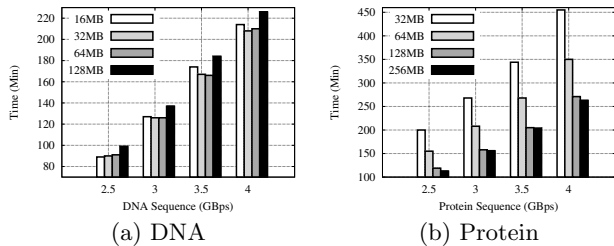
Figure 8: Tuning the size of R : 32MB for DNA ( |\Sigma|=4 ); 256MB for Protein ( |\Sigma|=20 )
